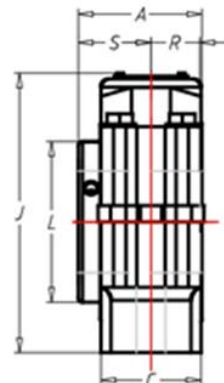
2 BOLT BASE
